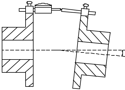
Angular Alignment
