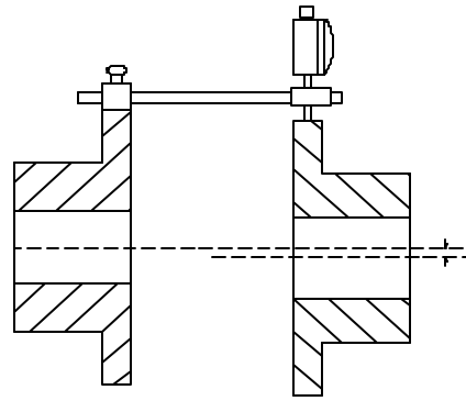
Parallel Alignment
